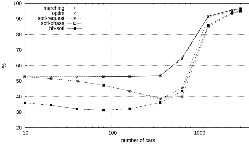
Fig. 3. Average stopped cars; 19 \times 19 grid
