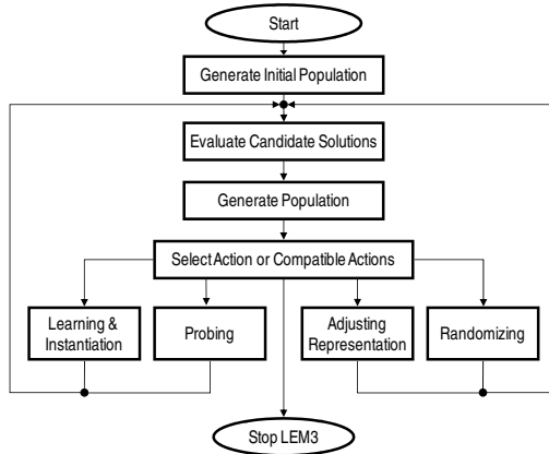
Fig. 1. Flowchart of the top level LEM3 algorithm
