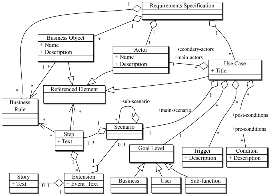
Fig. 1. Use-cases-based functional requirements specification model
