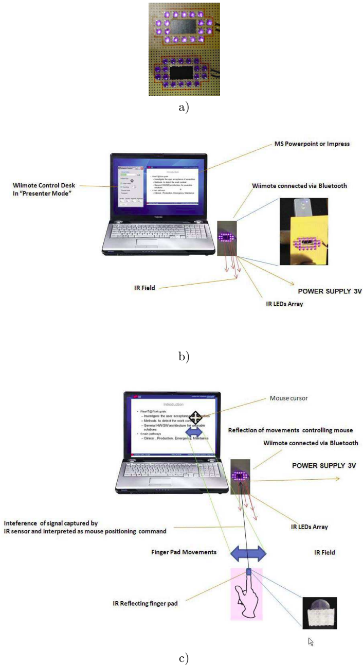
Fig. 1. Finger tracking with Wii Romote; a) IR LED array, b) Sensor setup for finger tracking, c) Finger tracking in action
