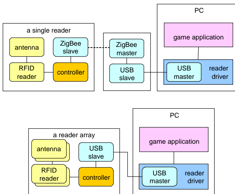
Fig. 4. Architectures of game boards with PCs
