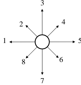
Fig. 9. Direction symbols in a chain code
