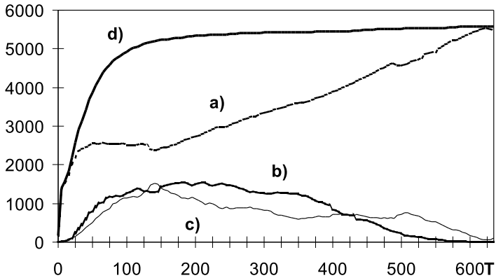
Fig. 9. Chart showing the number of agents in time ( T ). Variant with free agents (“un-employed”) the number of agents of type a^1 a), the number of agents of type a^2 b), the number of agents of type a^3 – free agents c), chart of the total number of agents of all types ( a^1, a^2, a^3 ) – d).
