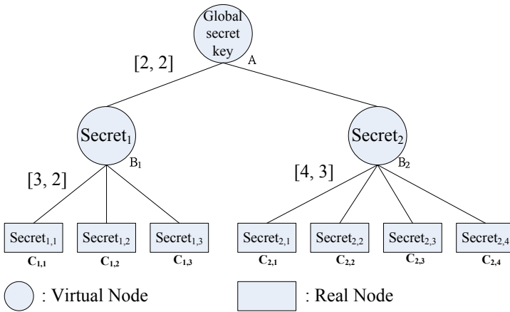
Fig. 1. Example of AKM
