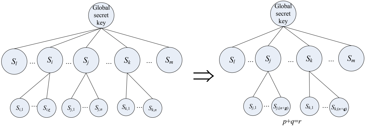
Fig. 2. Function Merge – merges S_i into S_j and S_k
