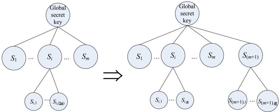
Fig. 3. Function Partition – partition of S_i into S_j and S_{m+1}
