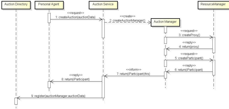
Figure 3. Agent interactions for initiating an auction
