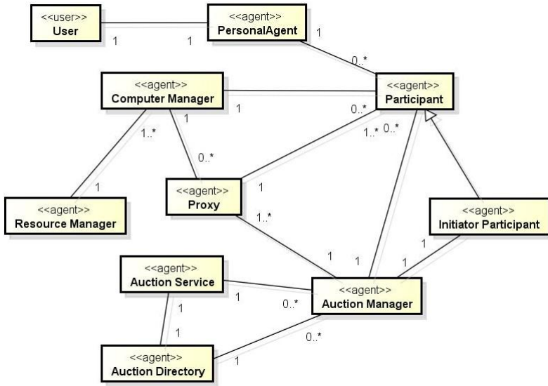
Figure 1. Relationships between users, agent types and auctions on the auction server
