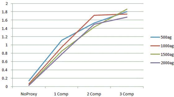
Figure 14. Throughput [no. of bids/ms]
