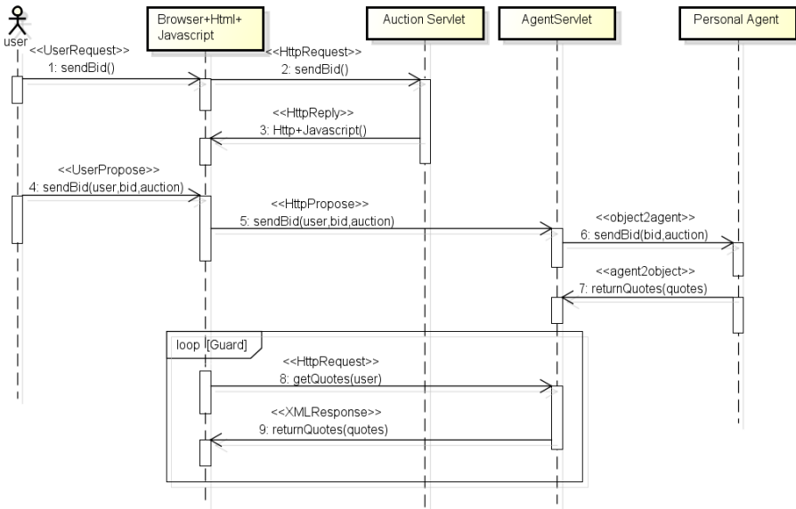
Figure 11. Participating in an auction
