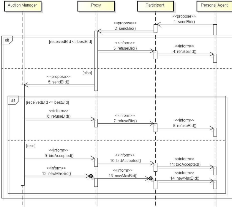
Figure 6. The bid submission protocol
