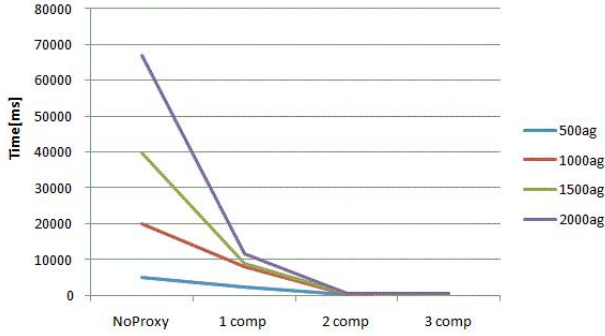
Figure 13. Latency [ms]
