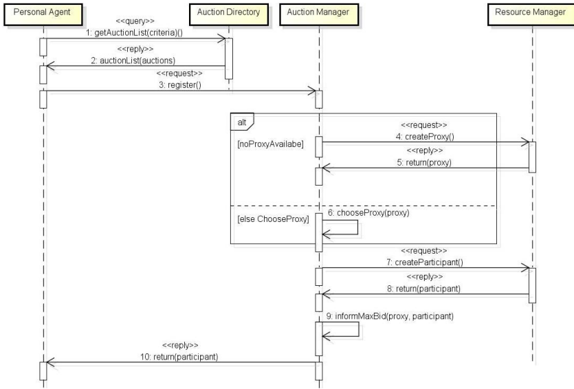
Figure 4. Searching for and joining an auction
