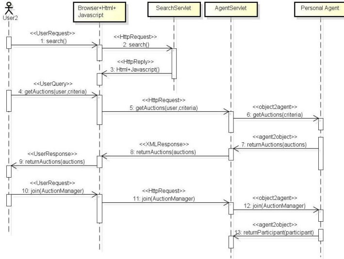
Figure 10. Searching and joining an auction
