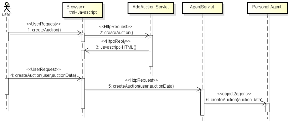
Figure 9. Initiation of an auction
