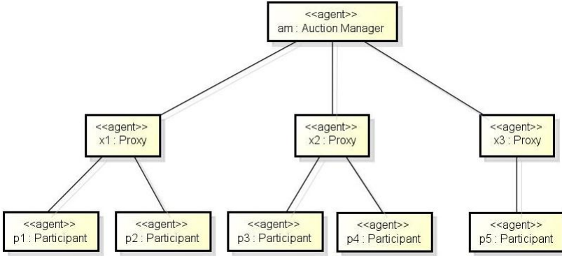
Figure 2. Relationships between Participant , Proxy , and Auction Manager agents involved in an auction on the auction server
