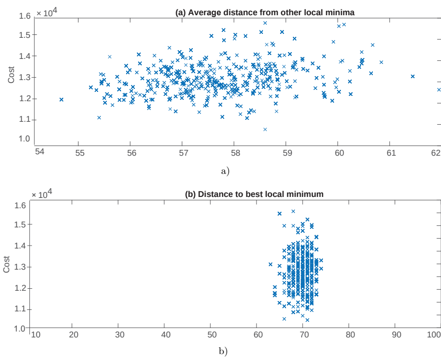
Figure 2. 2000 random 2-opt local minima for pr1002-x. Tour cost (vertical axis) is plotted against a) mean distance to the 1999 other local minima and b) distance to the global minimum.
