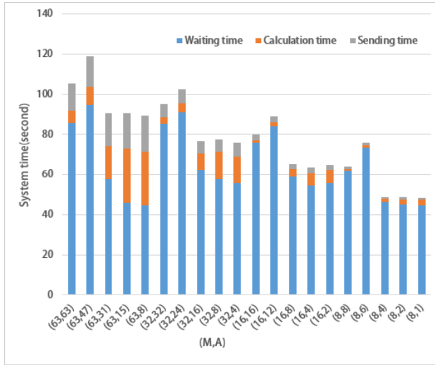
Figure 7. The system time allocation of the GAD-ADMM with different groups ( M ) and thresholds ( A )
