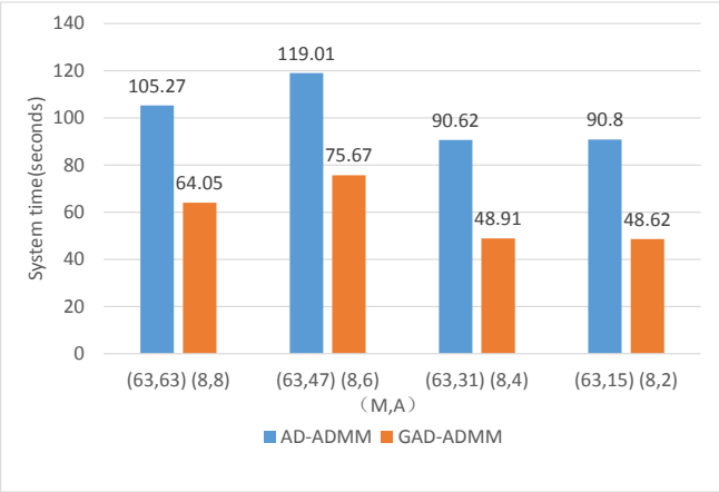
Figure 4. The system time cost of the AD-ADMM and the GAD-ADMM: A is the threshold and M is the number of groups
