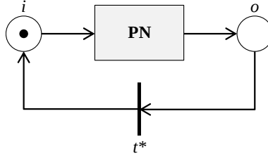
Figure 3. Example of extended Petri net
