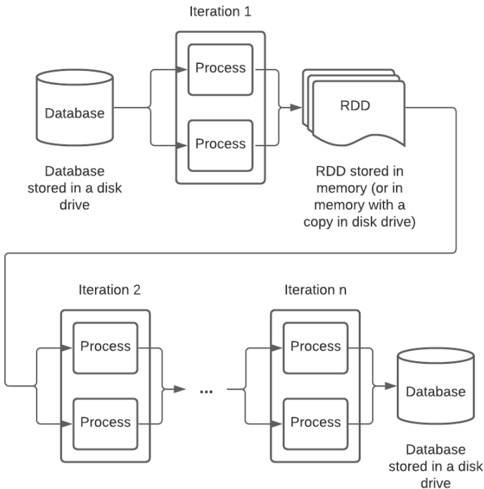
Figure 2. Working of RDDs in Apache Spark
