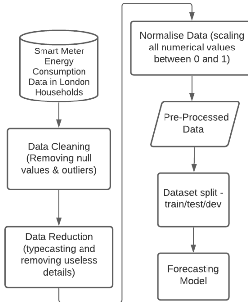
Figure 1. Flowchart of data pre-processing
