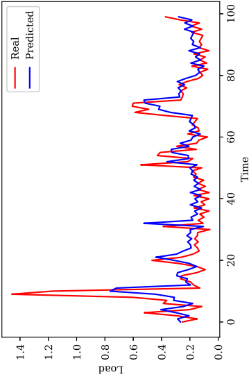
c) LSTM
