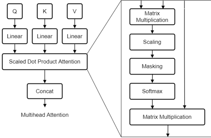
Figure 4. Mechanism of multihead self-attention layer
