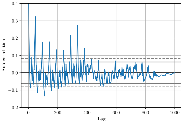
Figure 7. Self-Autocorrelation over 1000 timesteps for one house
