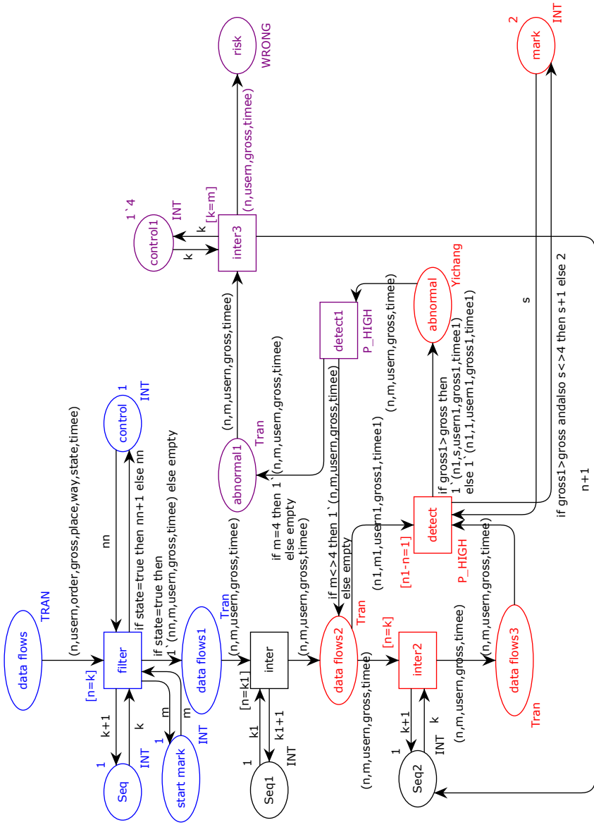
Figure 4. The Event Pattern model for the anomaly detection of the continuous increase of user payment amount
